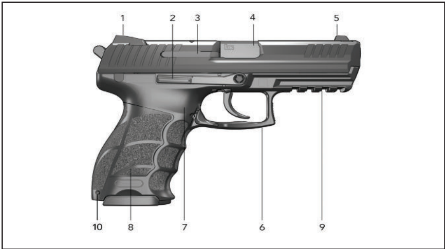
Figure 1 — P30 (right side view)
