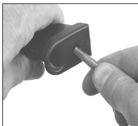
Figure 32 Depressing locking plate in floorplate
