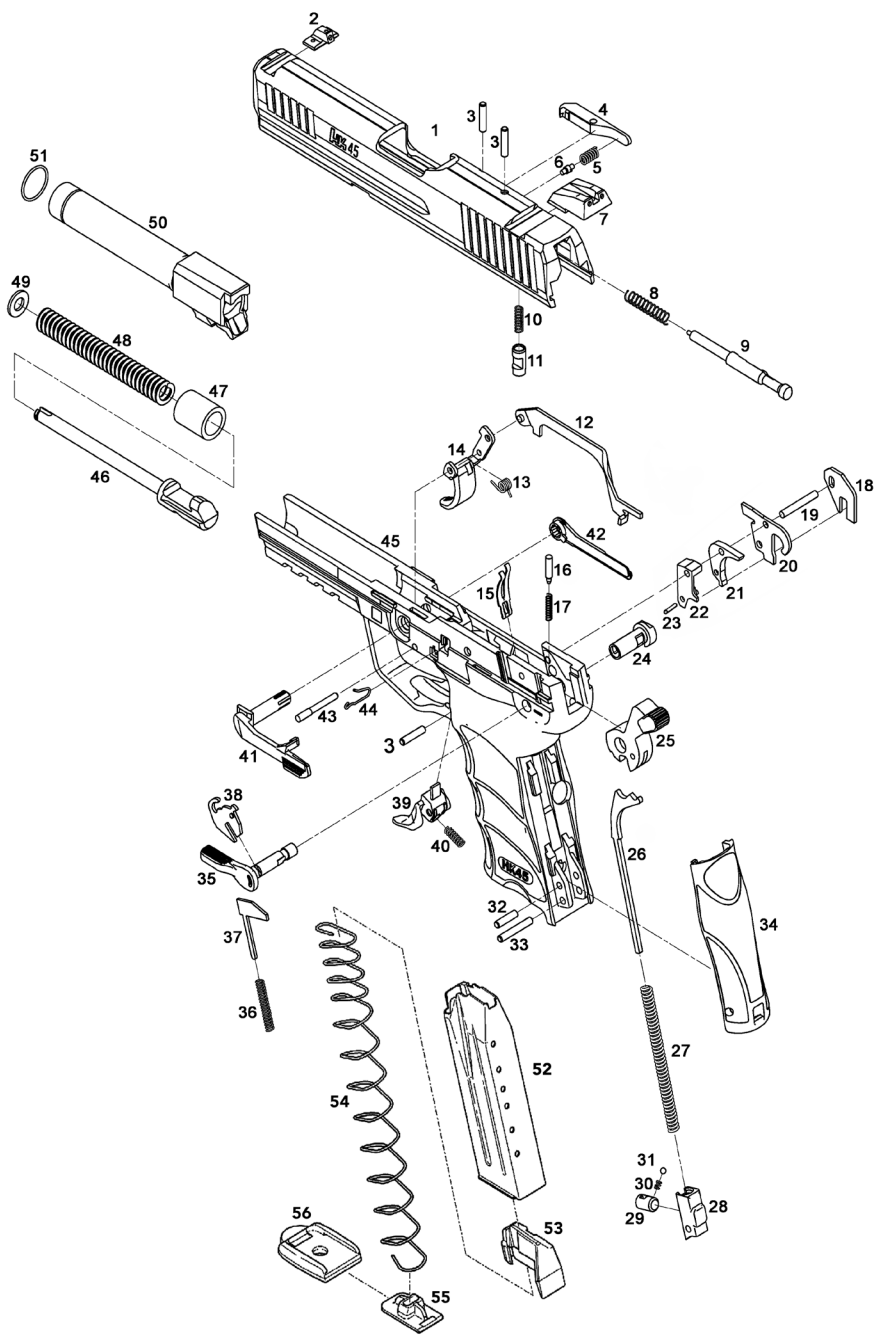
Figure 46 — HK45 Exploded Diagram
