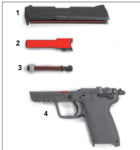
Figure 39 — Lubrication Points (in red)
