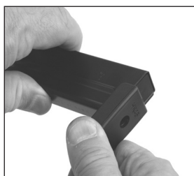
Figure 33 Slide the floorplate forward
