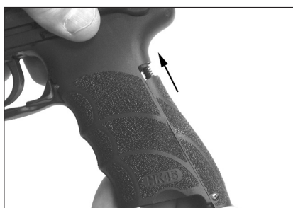
Figure 29 — Slide backstrap
