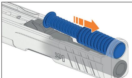
Figure 26 – Insert recoil spring assembly
