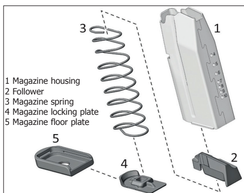
Figure 35 – Assemble magazine
