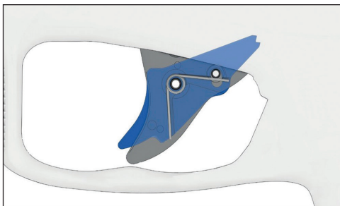
Figure 5 – Trigger safety
