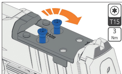
Figure 17 – Tighten screws
