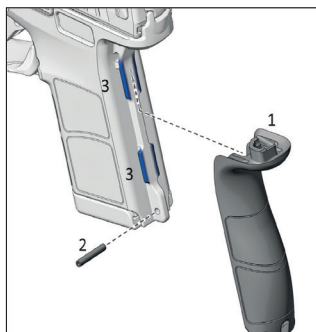
Figure 31 – Backstrap
