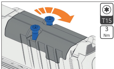
Figure 15 – Tighten screws
