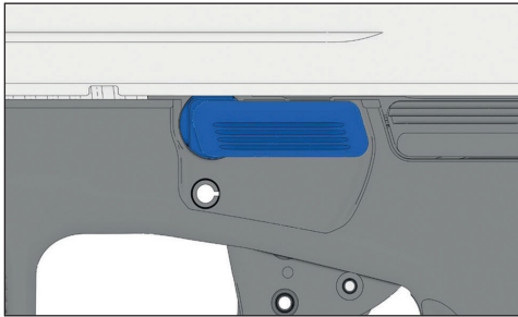
Figure 7 – Disassembly safety
