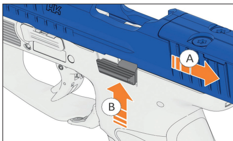
Figure 22 - Locking the slide to the rear
