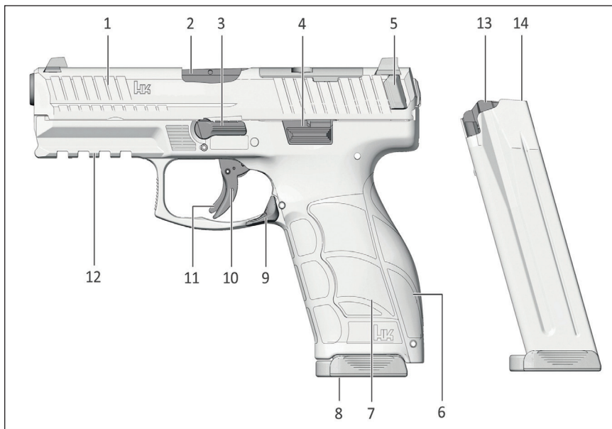
Figure 2 – VP9A1 Series (left side view)
