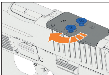
Figure 19 – Tighten screws
