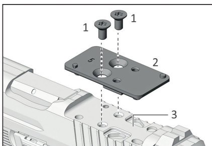
Figure 18 – Tighten screws
