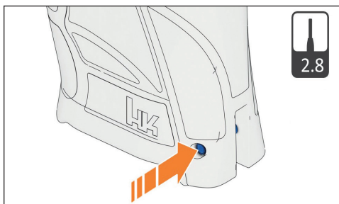
Figure 34 – Drive out clamping sleeve for backstrap
