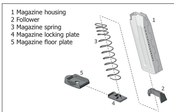
Figure 37 – Assemble magazine
