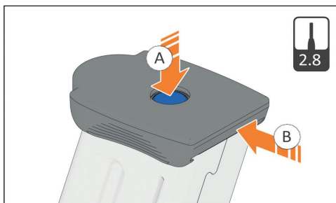
Figure 36 – Slide magazine floor plate forward
