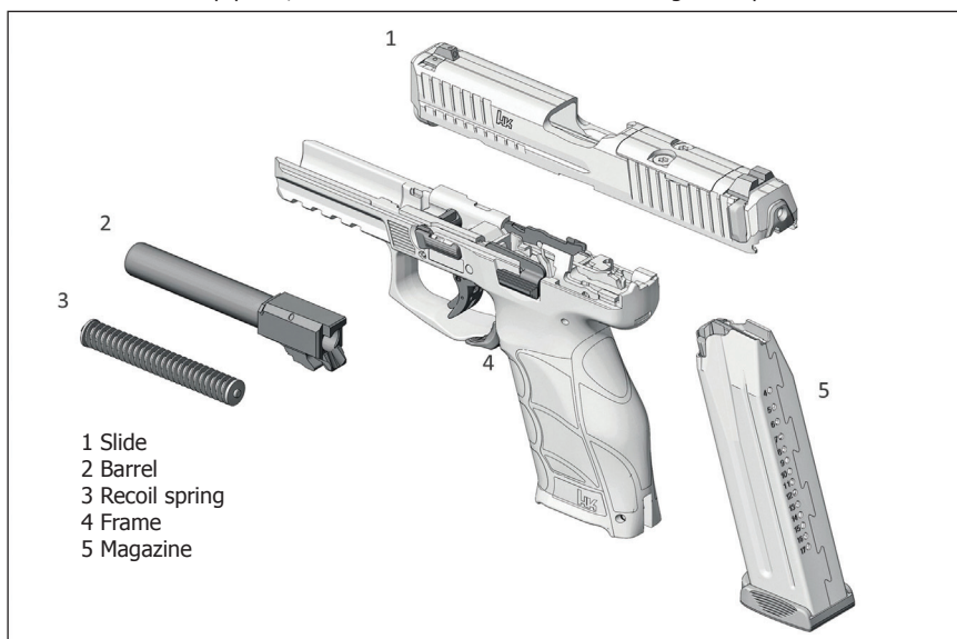
Figure 3 – VP9A1 Assembly Groups
