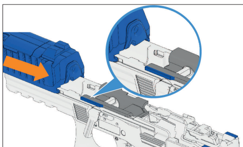
Figure 31 – Push slide over guide-rails
