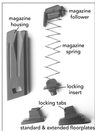
Fig. 24 – 10-rd. magazine components
