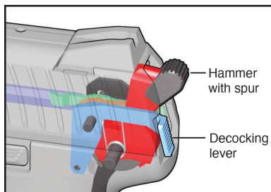
Figure 18 — V3 DA/SA firing mode
