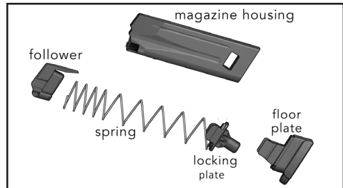
Figure 37 10-round magazine components
