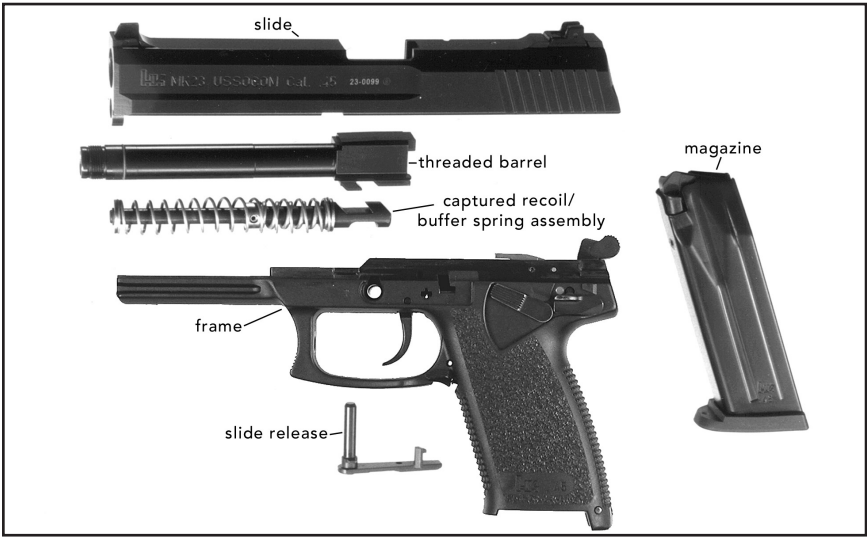
Figure 3 Major Assembly Groups
