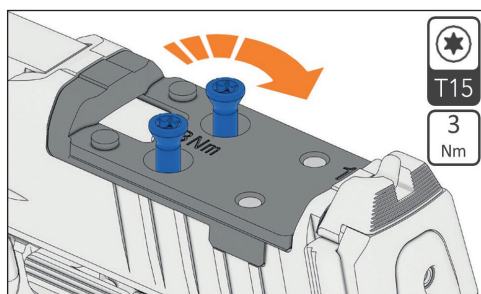
Figure 17 – Tighten screws
