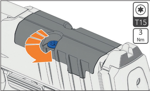
Figure 14 – Loosen screws
