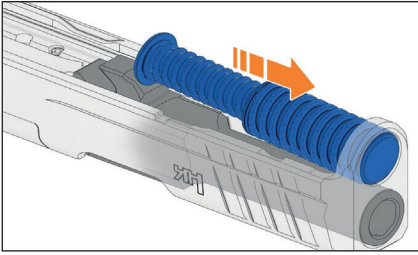
Figure 26 – Insert recoil spring assembly
