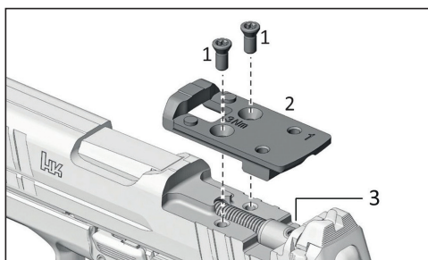
Figure 16 – Tighten screws
